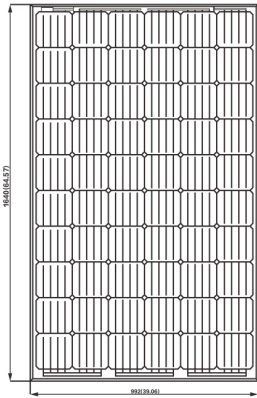
Dimension of PV Modules Unit: mm
