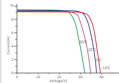
I-V characteristics at different temperature
