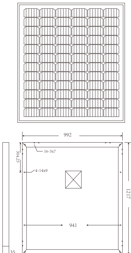
Dimension of PV Modules Unit: mm
