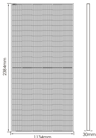
Dimension of PV Modules Unit: mm
