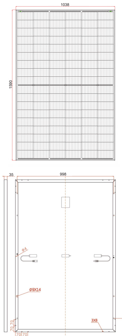
Dimension of PV Modules Unit: mm
