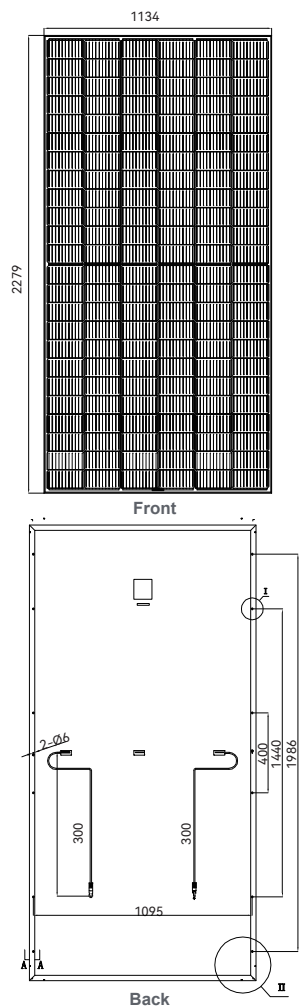
Dimension of PV Modules Unit: mm
