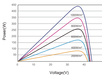
P-V CURVES OF PV MODULE(450W)
