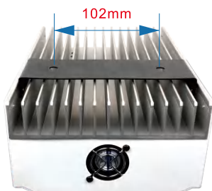
安装孔距— \varnothing 5 Mounting hole Size
