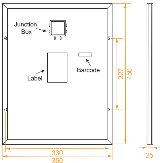
Dimension of PV Modules Unit: mm
