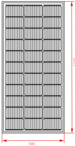
Dimension of PV Modules Unit: mm
