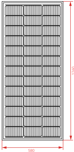
Dimension of PV Modules Unit: mm
