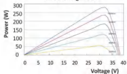
Power-Voltage Curve
