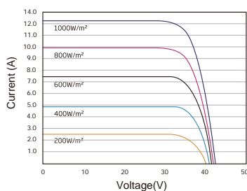
I-V CURVES OF PV MODULE(400W)
