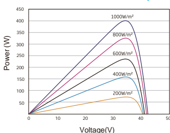
P-V CURVES OF PV MODULE(400W)
